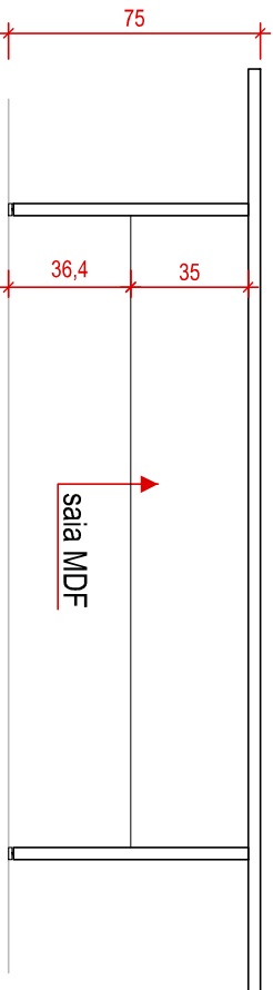
VISTA FRONTAL
