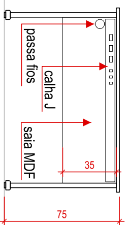
VISTA FRONTAL
