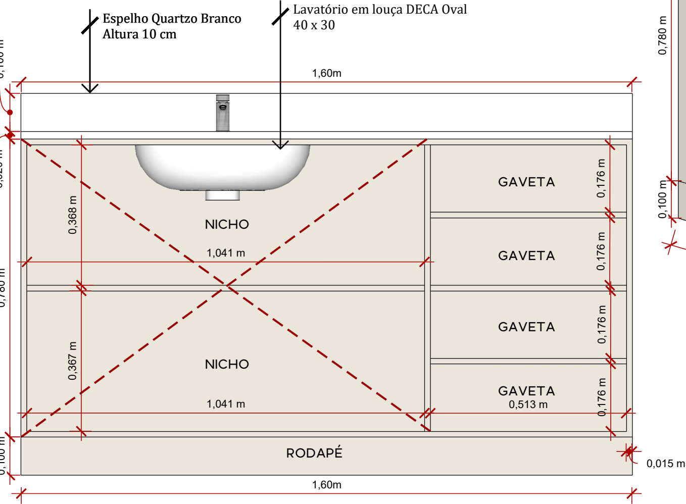
VISTA FRONTAL
