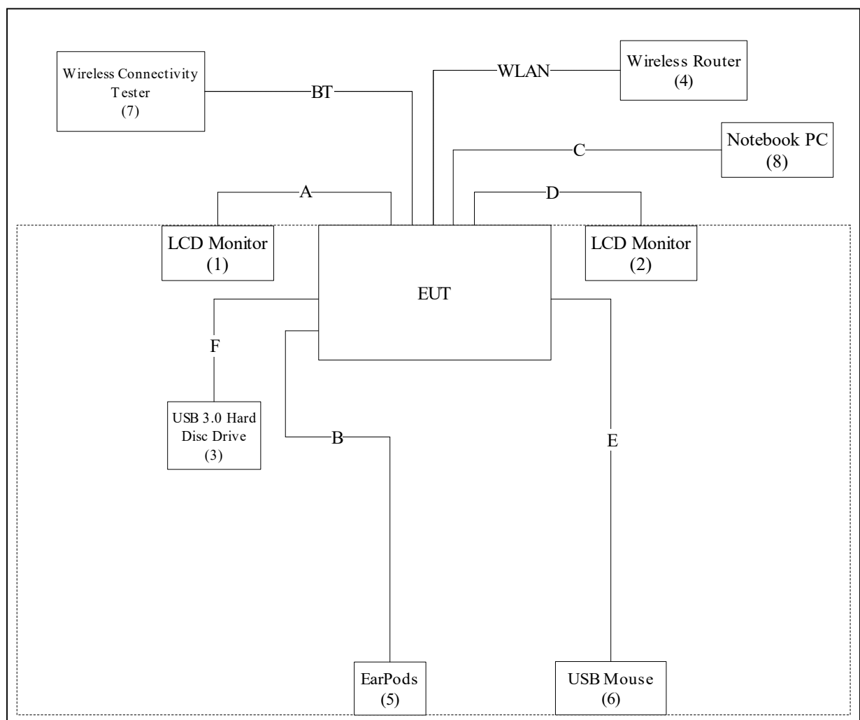
Connection Diagram
