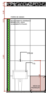
A.M.07 VISTA 3 Escala 1:25
