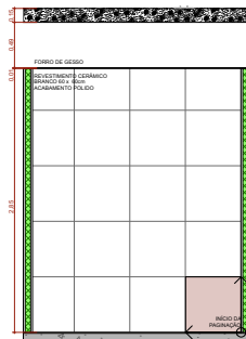
A.M.07 VISTA 1 Escala 1:25
