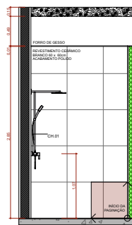
A.M.08 VISTA 1 Escala 1:25
