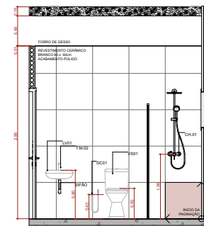
A.M.09 VISTA 4 Escala 1:25
