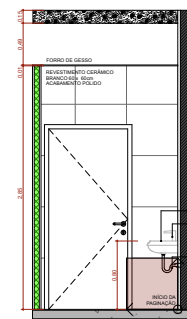
A.M.08 VISTA 4 Escala 1:25
