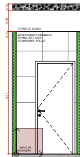
A.M.07 VISTA 2 Escala 1:25
