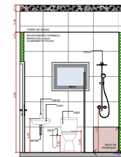
A.M.08 VISTA 2 Escala 1:25
