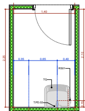
A.M.7 DML Escala 1:25
