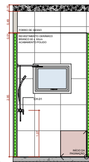
A.M.09 VISTA 1 Escala 1:25
