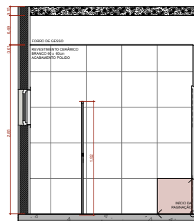
A.M.09 VISTA 3 Escala 1:25
