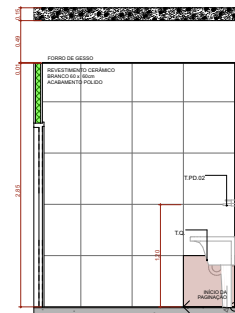
A.M.07 VISTA 4 Escala 1:25
