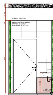
A.M.09 VISTA 2 Escala 1:25
