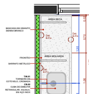
BPC.180d Escala 1:20
