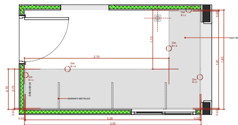
BPC.330de Escala 1:20
