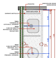
BPC.160d Escala 1:20
