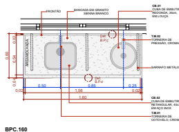
BPC.160 Escala 1:20
