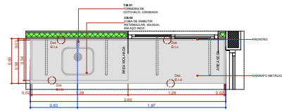
BPC.260d Escala 1:20
