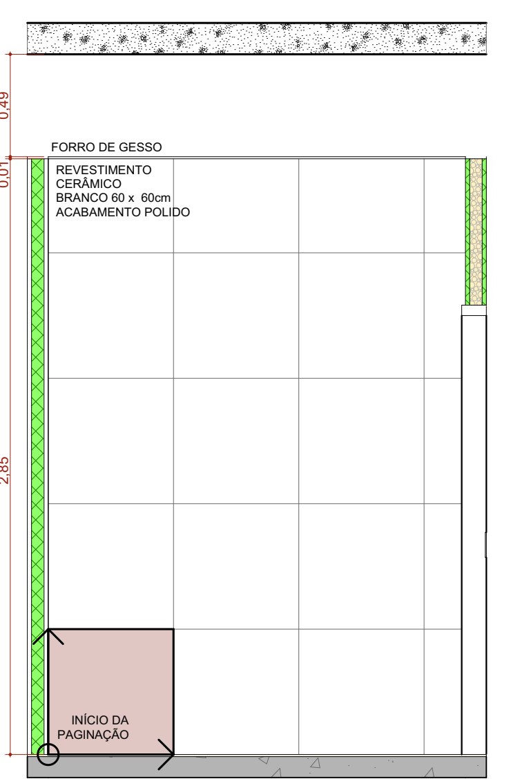
A.M.08 VISTA 01
