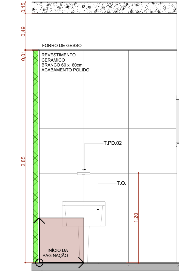
A.M.13 VISTA 04
