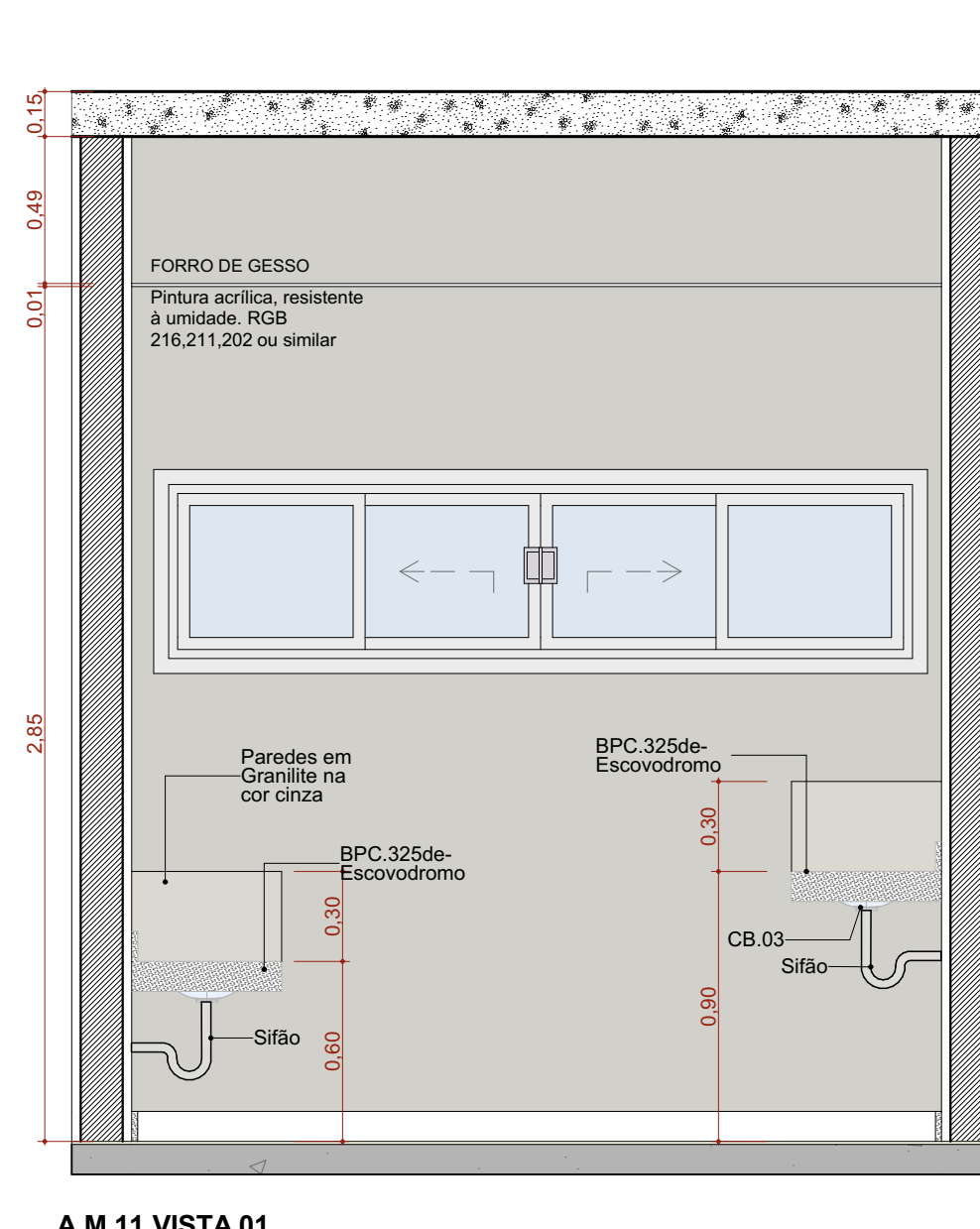
A.M.11 VISTA 01
