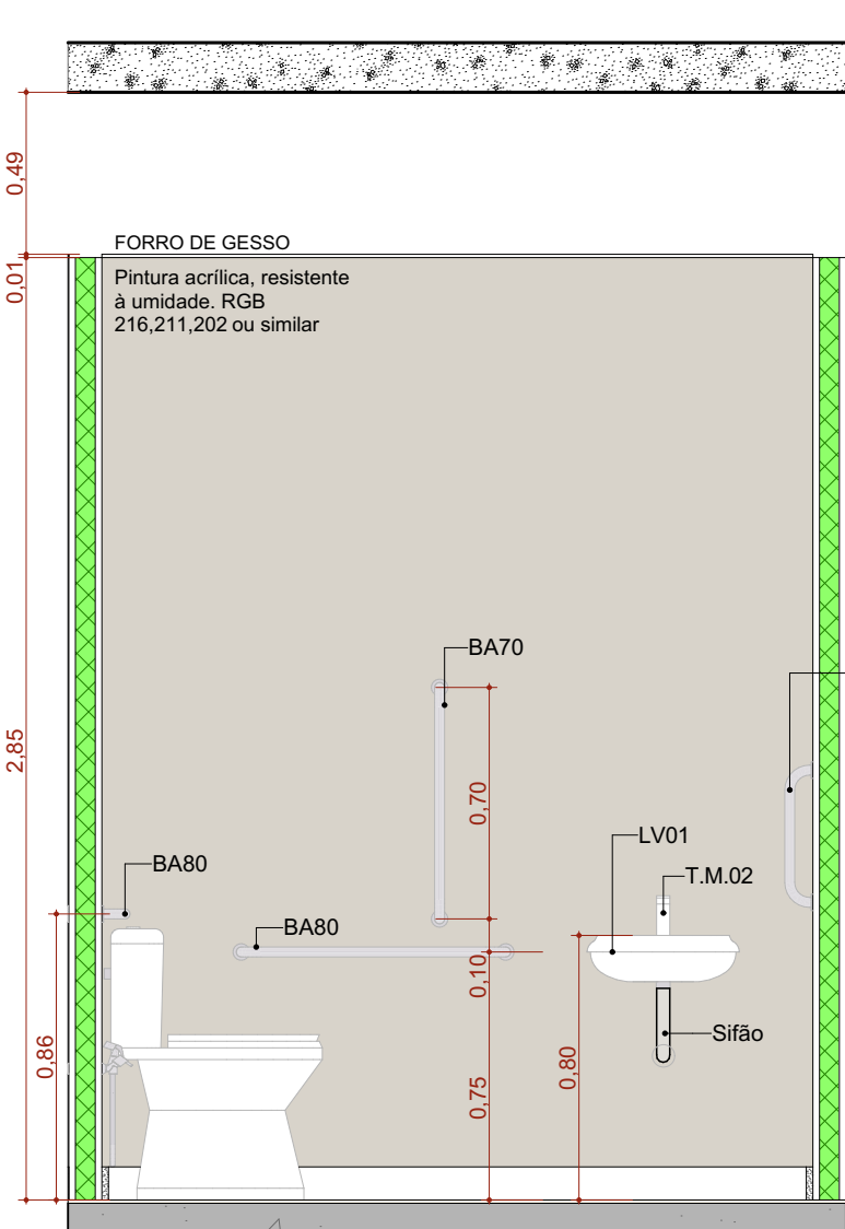
A.M.07 VISTA 04
