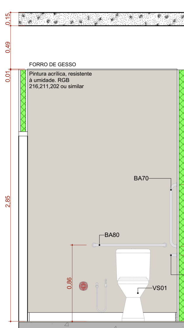
A.M.07 VISTA 03
