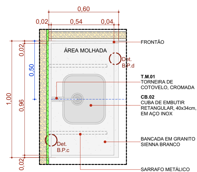
BPC.100d Escala: 1:20
