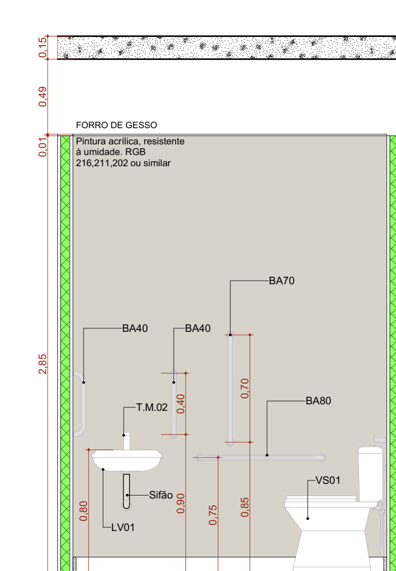
A.M.12 VISTA 04
