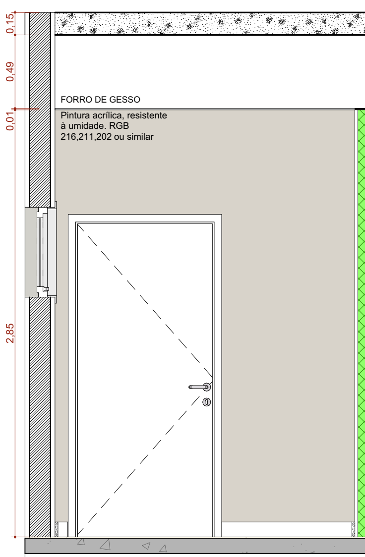
A.M.10 VISTA 04
