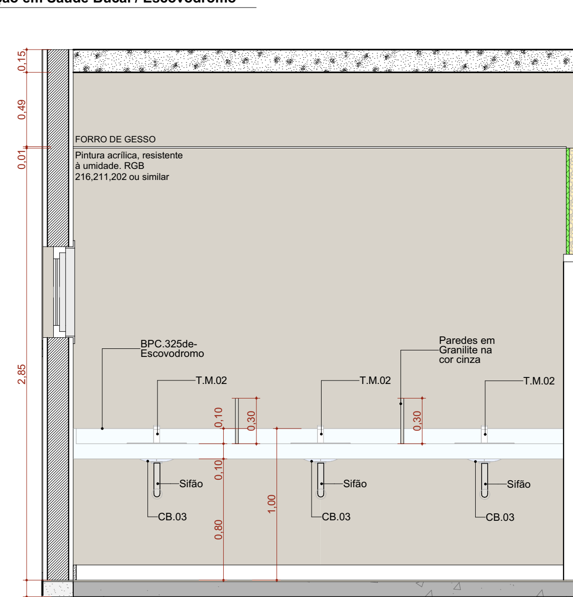
A.M.11 VISTA 03
