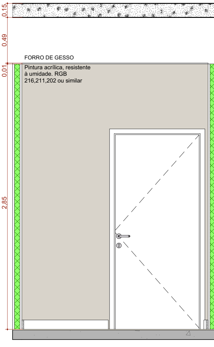
A.M.09 VISTA 02
