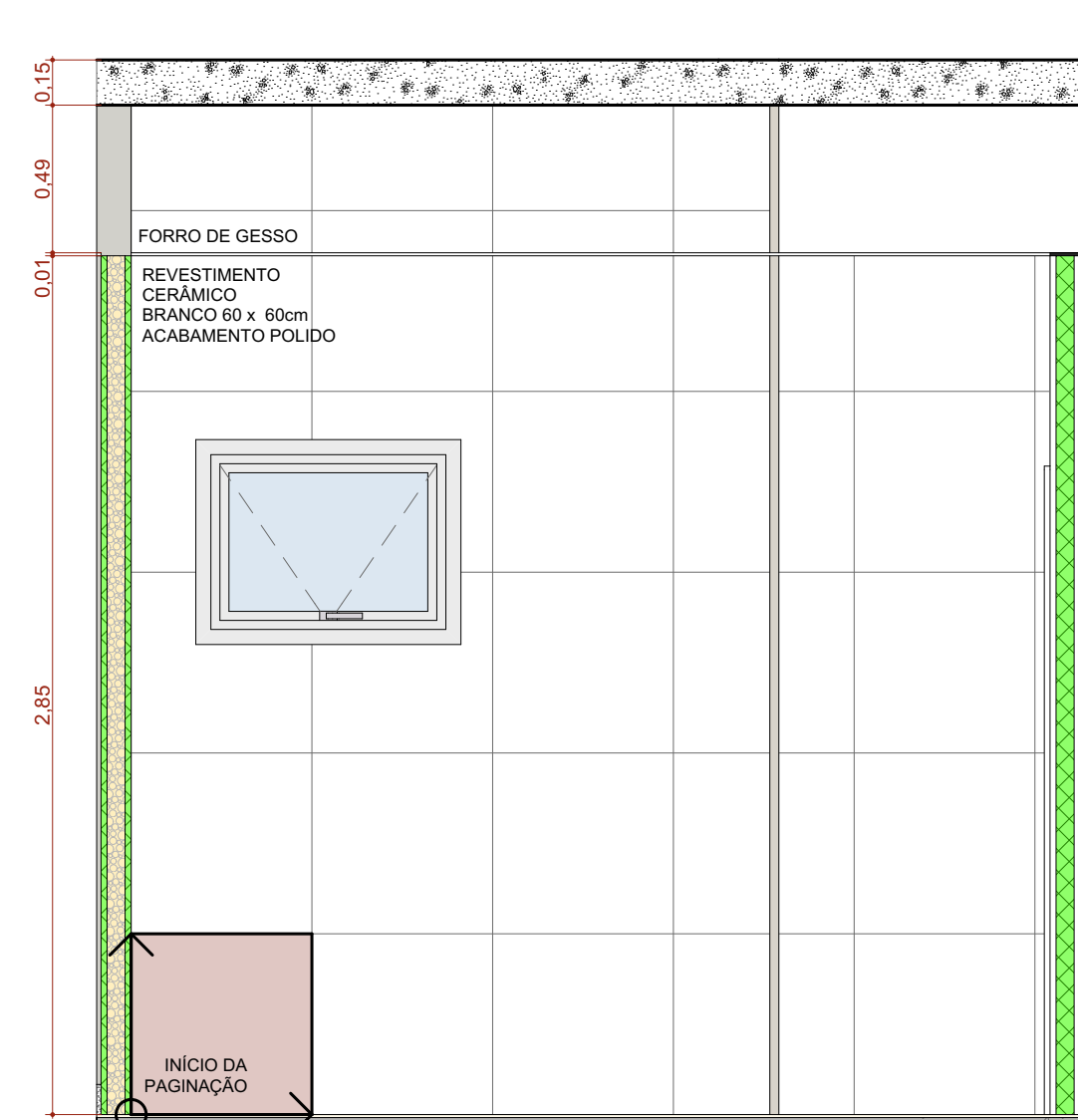
A.M.13 VISTA 01
