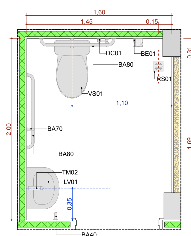
A.M.11 Sanit. Cons. Ind. 1 Escala: 1:25
