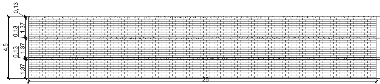
Vista Frontal
