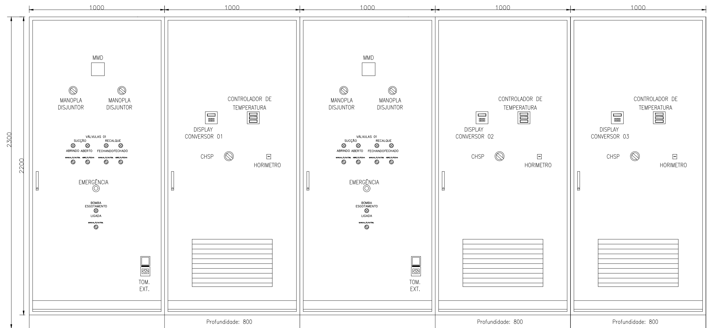
VISTA FRONTAL
